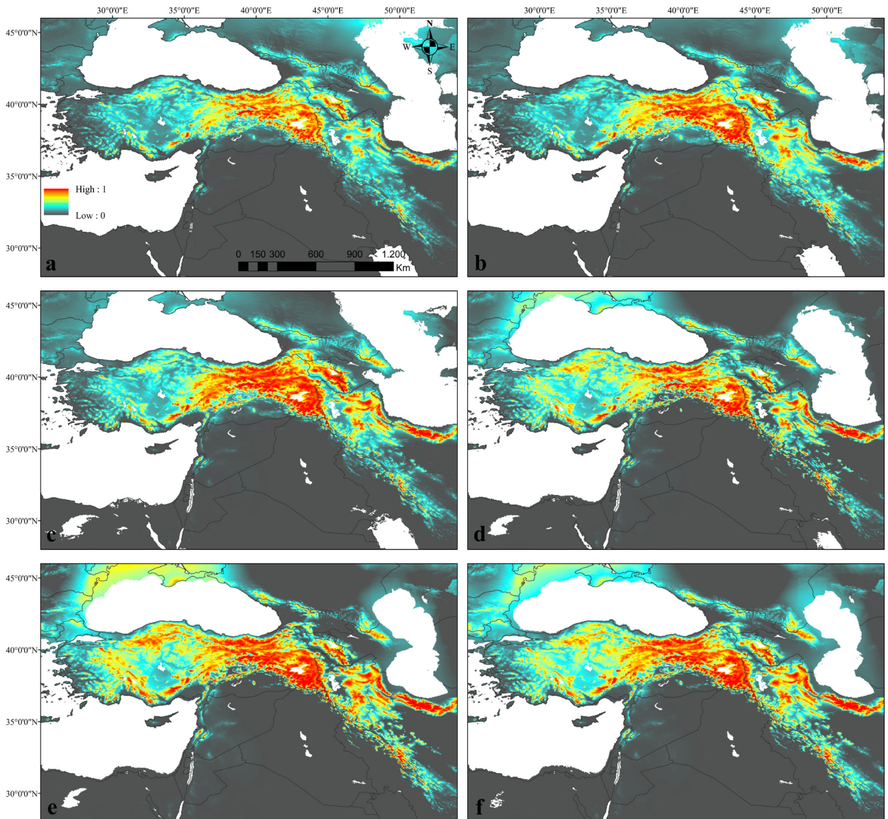
Figure 2. Bioclimatic suitability under the present and past bioclimatic conditions for Noccaea vesicaria : a) Present (1979–2013); b) Late Holocene, Meghalayan (4.2–0.3 ka); c) Mid-Holocene, Northgrippian (8.326–4.2 ka); d) Early Holocene, Greenlandian (11.7–8.326 ka); e) Younger Dryas Stadial (12.9–11.7 ka); f) Bølling-Allerød (14.7–12.9 ka). Note that the coastlines for past time periods differ from the present (more pronounced especially during colder time periods, e.g., Last Glacial Maximum) and also that the present borders of lakes are shown for past time periods.
