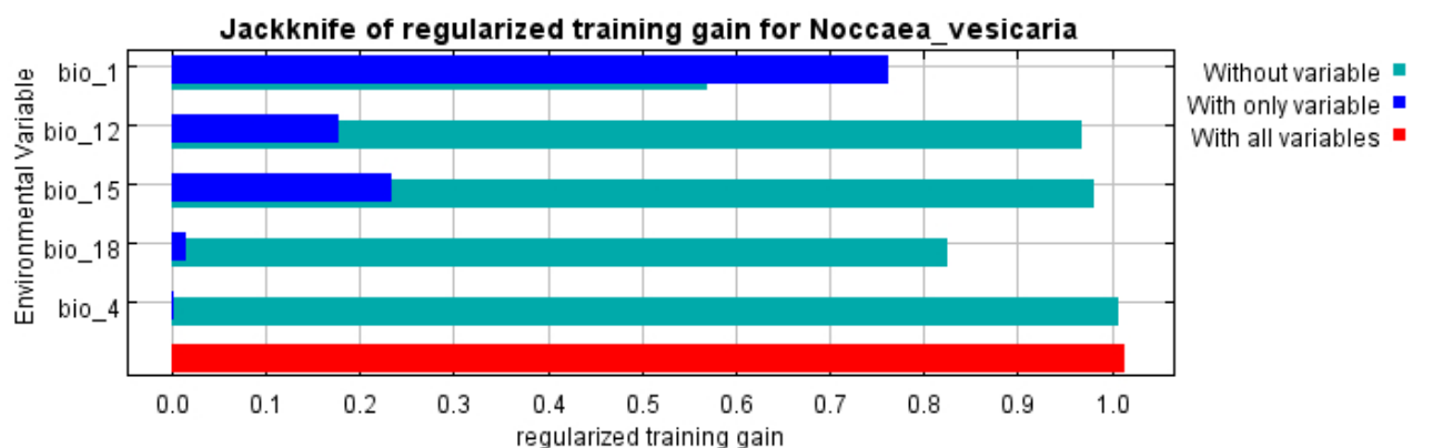
Figure S2. The results of the jackknife test of variable importance. Without variable: Each variable is excluded in turn and a model is created with the remaining variables. With only variable: a model is created using each variable in isolation. With all variables: a model is created using all variables (see for further details, Phillips 2021).
