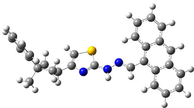
Figure 6. Calculated optimise structure of the title compound.
