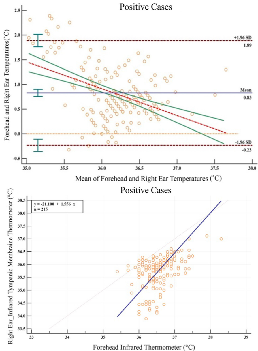
FIGURE 1 Bland–Altman plots and Passing–Bablok regression lines of temperature of forehead infrared thermometer and right infrared tympanic membrane thermometer in positive cases (n = 215) [Colour figure can be viewed at wileyonlinelibrary.com]
