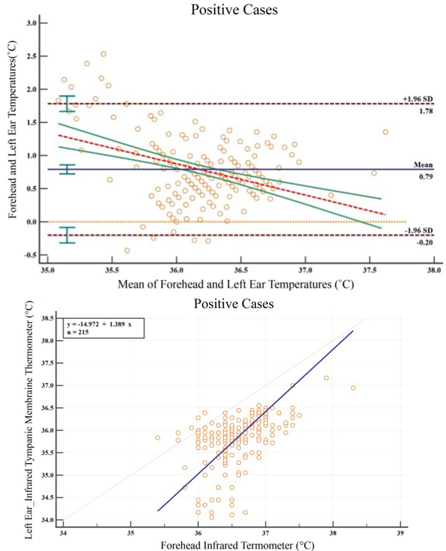
FIGURE 2 Bland–Altman plots and Passing–Bablok regression lines of temperature of forehead infrared thermometer and left infrared tympanic membrane thermometer in positive cases ( n = 215 ) [Colour figure can be viewed at wileyonlinelibrary.com ]
