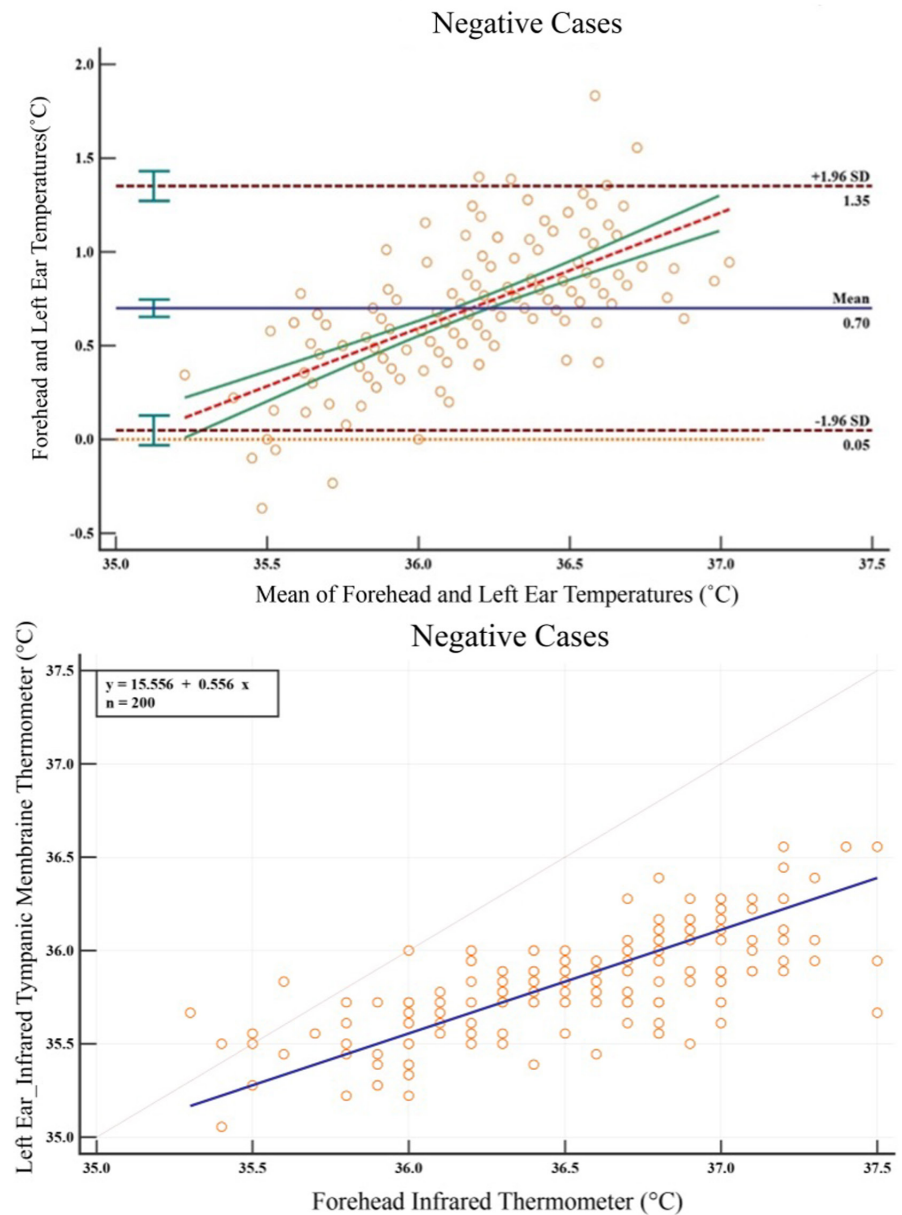
FIGURE 6 Bland–Altman plots and Passing–Bablok regression lines of temperature of forehead infrared thermometer and left infrared tympanic membrane thermometer in negative cases ( n = 200 ) [Colour figure can be viewed at wileyonlinelibrary.com ]
