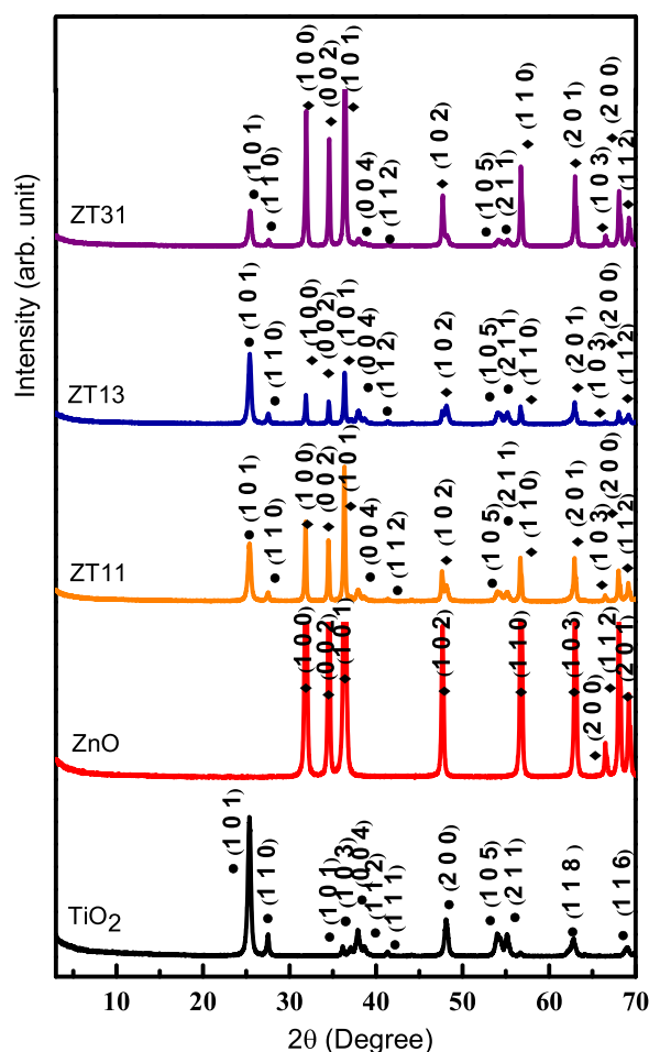
Fig. 1. XRD diffractograms \text{TiO}_2 , ZnO and ZnO/ \text{TiO}_2 binary oxides ZT11, ZT13 and ZT31. (• \text{TiO}_2 , ♦ ZnO).
