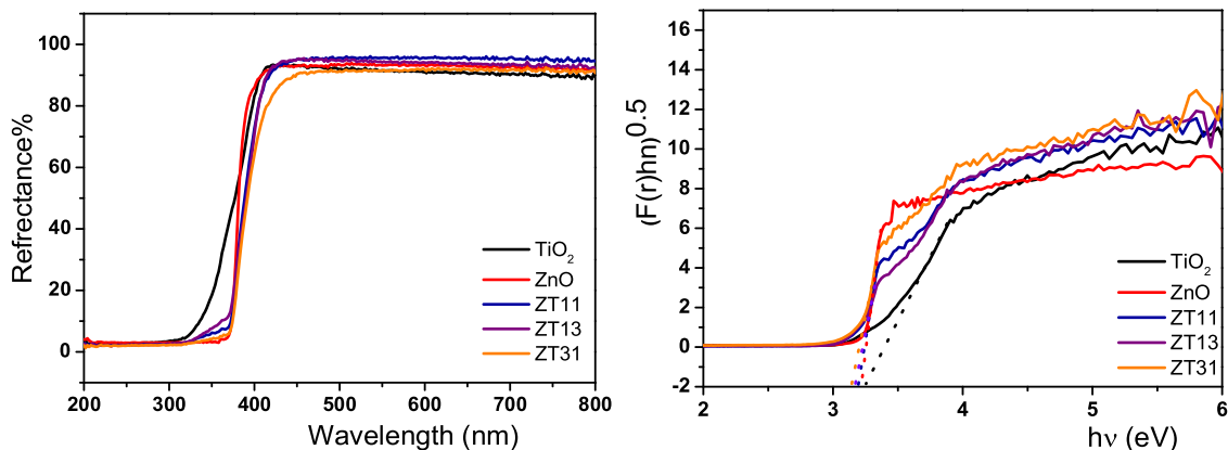
Fig. 5. UV-vis diffuse reflectance spectra A: \text{TiO}_2 , \text{ZnO} and \text{ZnO/TiO}_2 binary oxides ZT11, ZT13 and ZT31 and B: respective Tauc plots.
