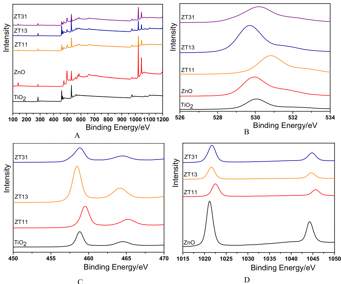
Fig. 3. XPS spectra of \text{TiO}_2 , \text{ZnO} and \text{ZnO/TiO}_2 binary oxides A: survey spectra of ZT11, ZT13 and ZT31, B: O 1s, C: Ti 2p, D: Zn 2p.
