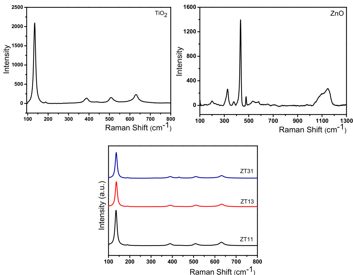
Fig. 4. Raman spectra of \text{TiO}_2 , \text{ZnO} and \text{ZnO/TiO}_2 binary oxides ZT11, ZT13 and ZT31.
