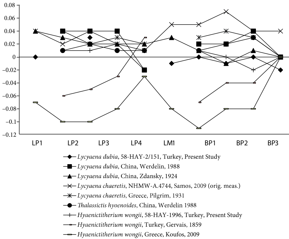
Figure 3. Logarithmic ratio diagram comparing the teeth of L. dubia , L. chaeretis , T. hyaenoides , and H. wongii from various localities.
