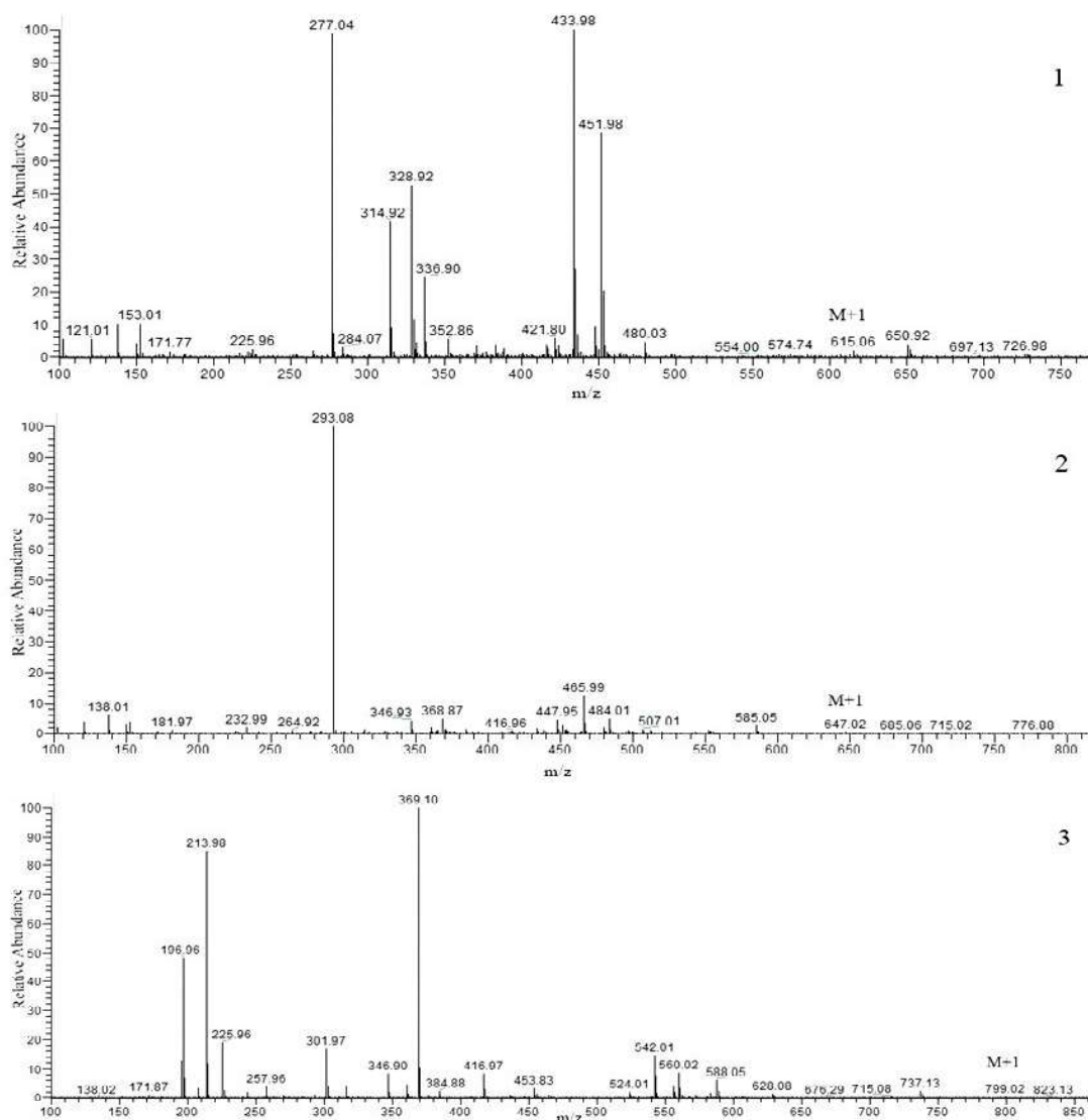
Fig. 1: LC-MS spectra of the copper (II) complexes.
