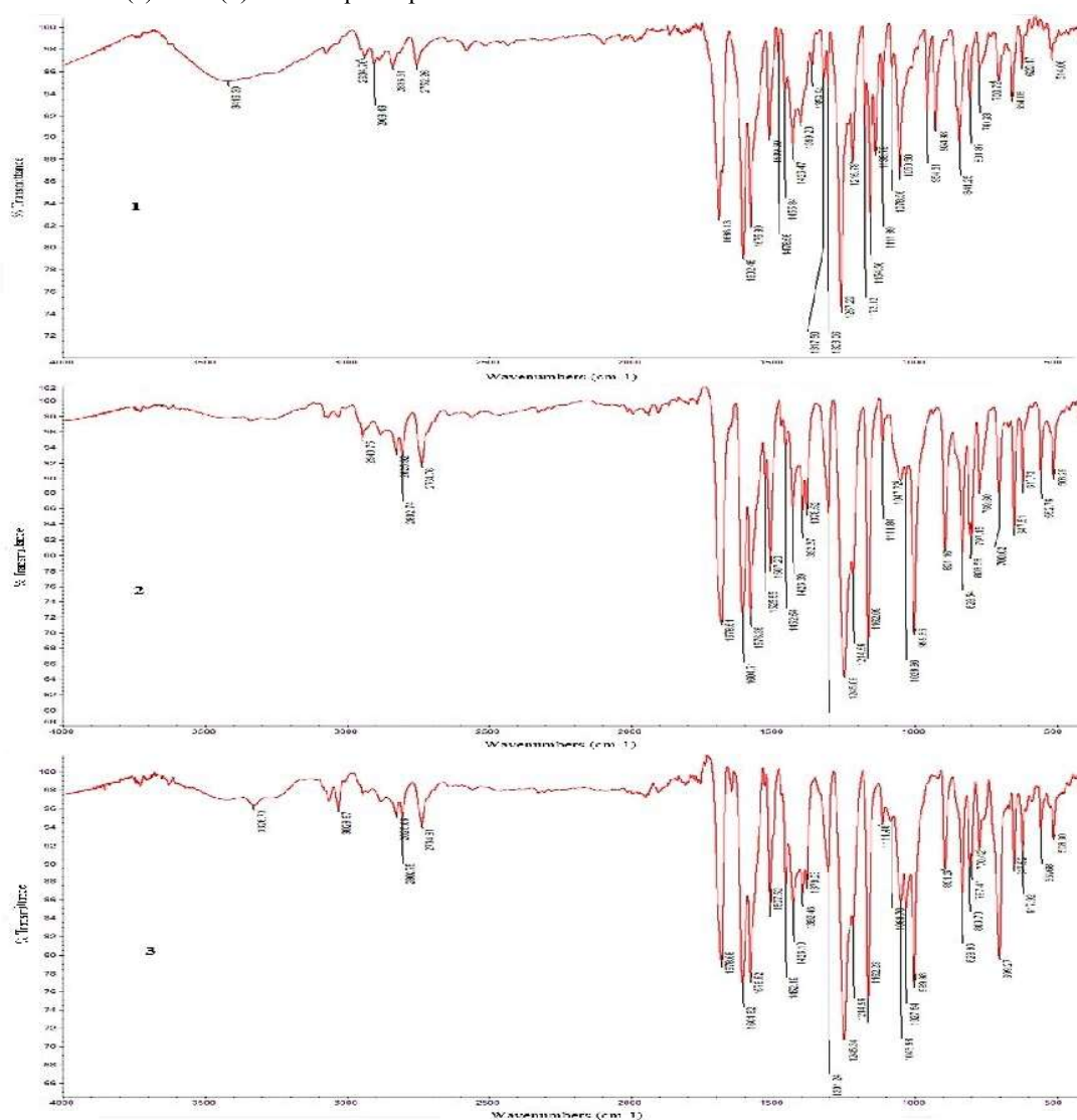
Fig. 2: FT-IR spectra of the copper (II) complexes.
