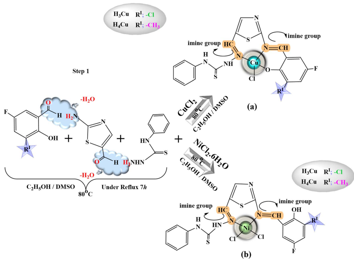
Fig. 2 General procedure for the heterocyclic thiosemicarbazone (a) Cu complexes ( \text{H}_3\text{Cu} , \text{H}_4\text{Cu} ) and Ni complexes ( \text{H}_3\text{Ni} , \text{H}_4\text{Ni} ).
