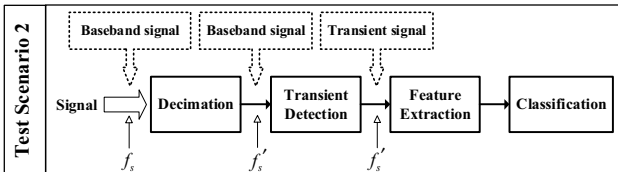
Fig. 5. Test Scenario 2: Decimating baseband signals.
