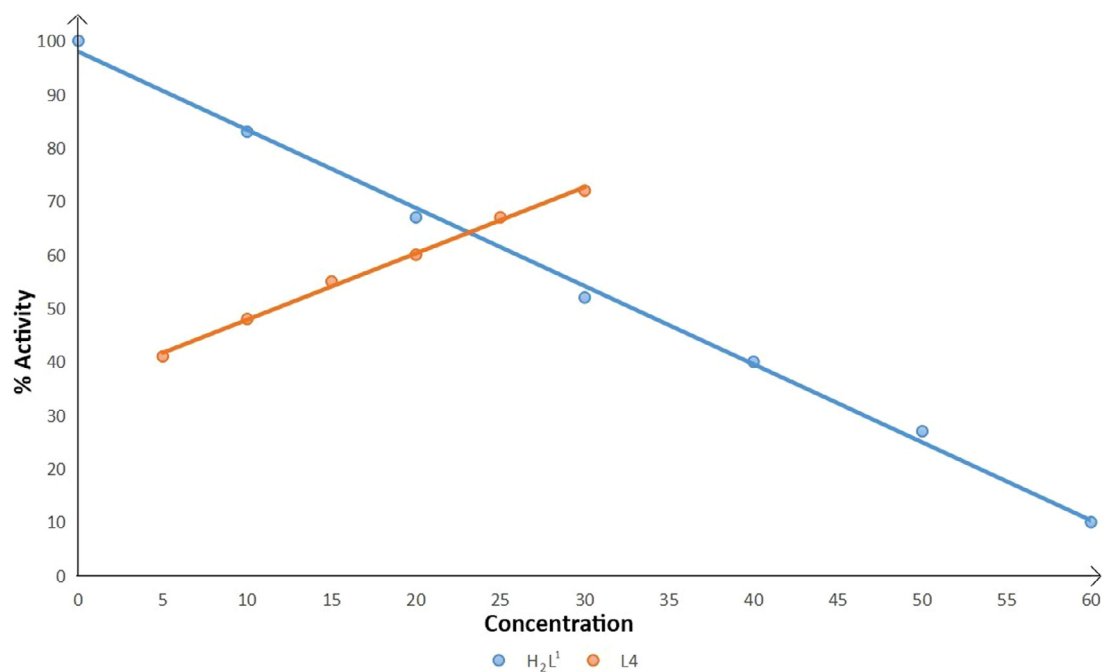
Fig. 3. % Activity - concentration (μM) graph of the H_2L^1 and L^4 for yeast GR.
