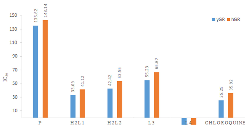
Fig. 4. Bar graph of IC 50 (μM) values of the compounds for GRs.
