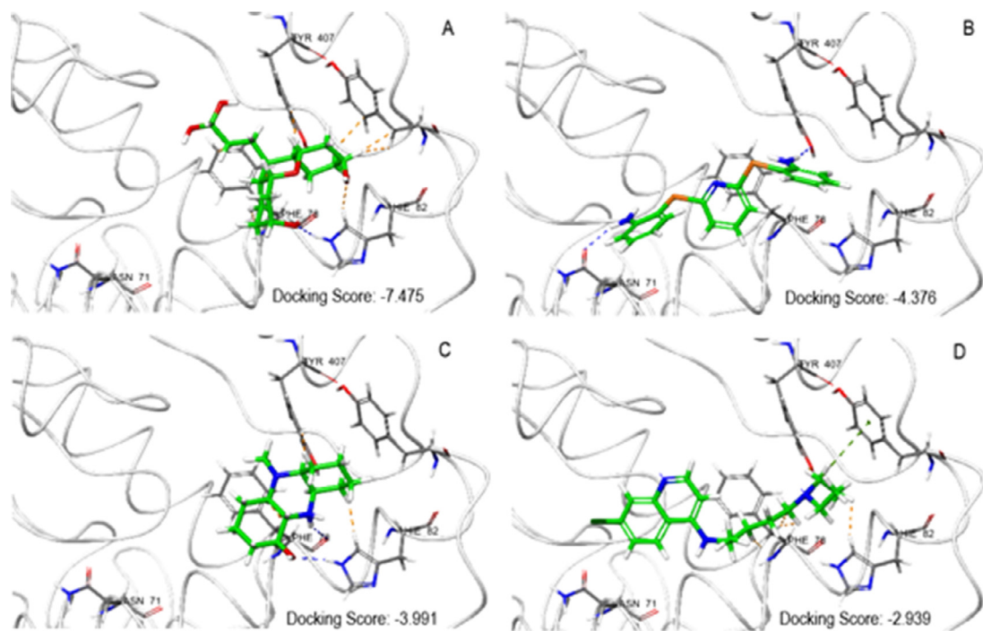
Fig. 5. Human GR (ID:1XAN) structural cartoon models of the ligands with docking score, (A) xantane, (B) 2,2'-(pyridine-2,6-diylsulfanediy)l)dianiline (C) pyocyanin (D) chloroquine.
