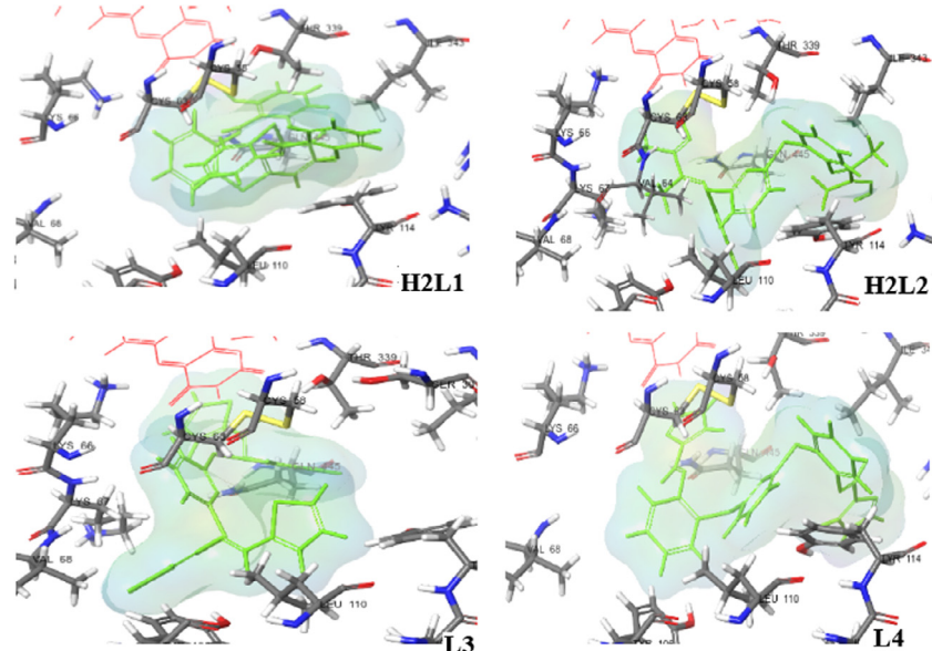
Fig. 7. Molecular docking of the Schiff bases at the active site of GR (PDB:1GRA). Solid surface spans the volume of the Schiff base. FAD (red), Schiff base (green).
