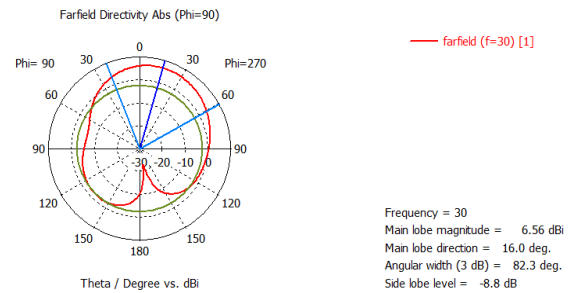
Figure 7. Radiation patterns for the square microstrip patch antenna without slots.
