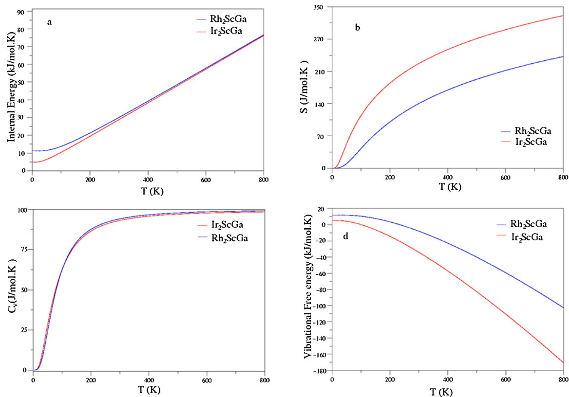
Fig. 6. The temperature dependence of (a) Internal energies (b) Entropies (c) Constant volume heat capacities and (d) Vibrational free energies of X_2\text{ScGa} ( X = \text{Ir} and \text{Rh} ) alloys.
