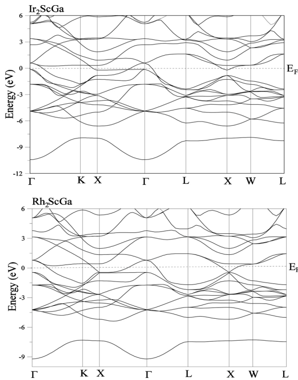
Fig. 2. Electronic band structures of X_2\text{ScGa} ( X = \text{Ir} and \text{Rh} ) alloys along the selected lines of high symmetry.
