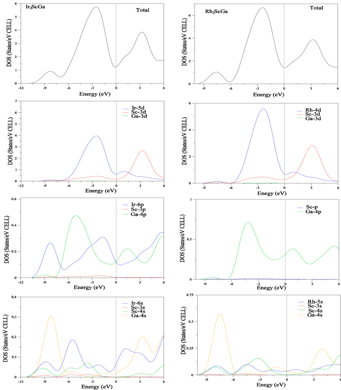
Fig. 3. The electronic total and partial density of states of X_2\text{ScGa} ( X = \text{Ir} and \text{Rh} ) alloys.
