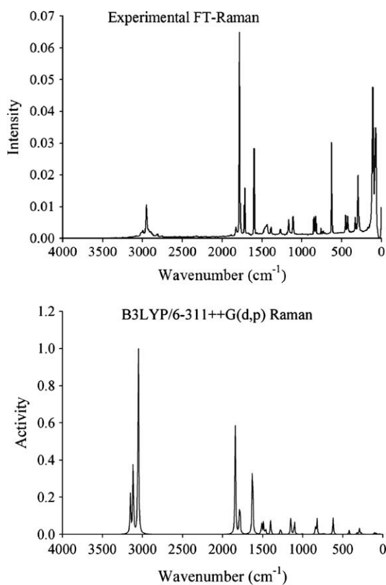
Fig. 2. Experimental and theoretical Raman spectra of 2,3DBrNMM.
