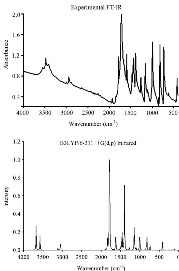
Fig. 3. Experimental and theoretical Infrared spectra of 2,3DBrNMM.
