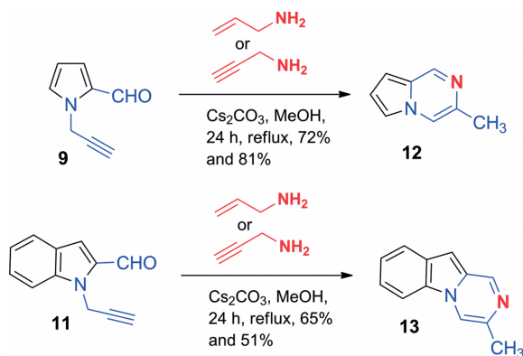
Scheme 5. Cyclization reactions of 9 and 11 with allylamine and propargylamine.
