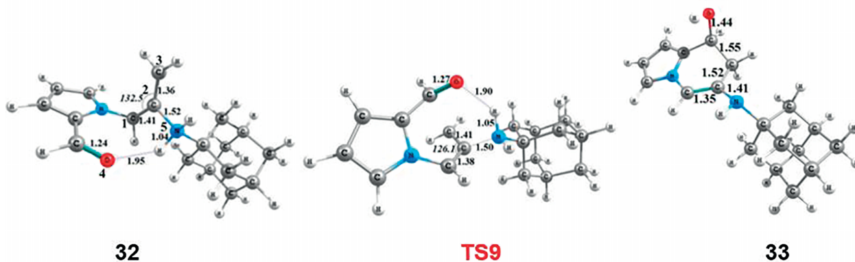
Figure 11. Optimized geometries of the stationary points of the second step for the formation of 34 at CPCM/B3LYP/6-31+G(d,p)//B3LYP/6-31+G(d,p) level in methanol. Distances are given in angstroms, angles are given in degrees.
