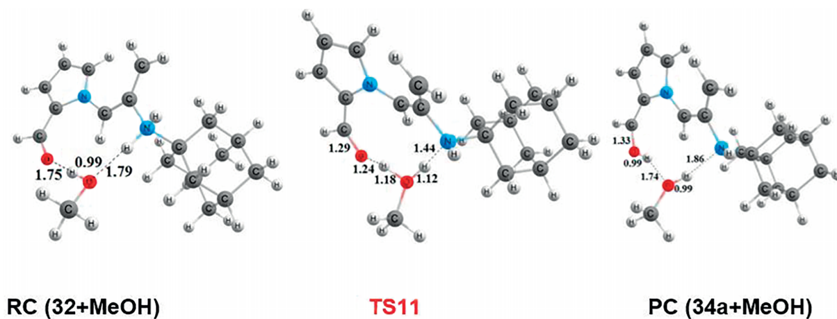
Figure 12. Optimized geometries of the stationary points for the formation of 34a at CPCM/B3LYP/6-31+G(d,p)//B3LYP/6-31+G(d,p) level in methanol. Distances are given in angstroms.
