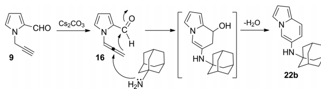
Scheme 8. Mechanism for the formation of 22a (and 22b ).
