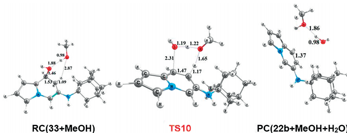
Figure 14. Optimized geometries of the stationary points for the formation of indolizine derivative 22b at CPCM/B3LYP/6-31+G(d,p)//B3LYP/6-31+G(d,p) level in methanol. Distances are given in angstroms.
