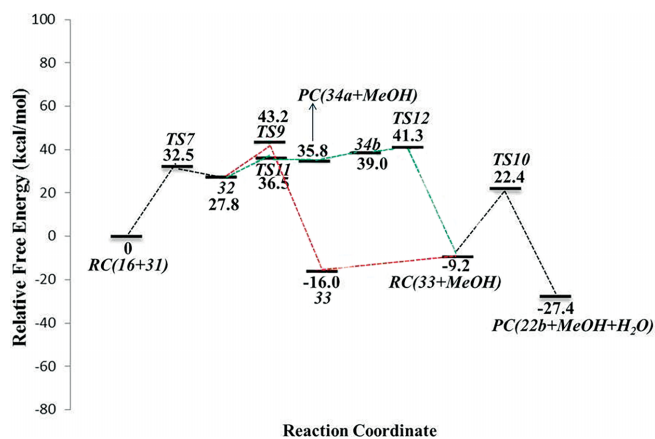
Figure 10. Potential energy profile and relative Gibbs free energies (kcal/mol) in methanol related to formation of indolizine derivative 22b at CPCM/B3LYP/6-31+G(d,p)//B3LYP/6-31+G(d,p) level. Black, common steps; red, path 1; green, path 2.
