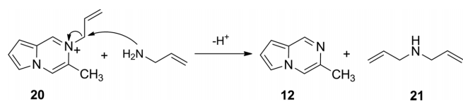
Scheme 6. Mechanism for the formation of 21 .
