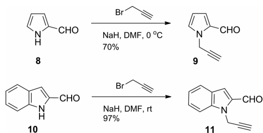
Scheme 1. Propargylation of pyrrole and indole aldehyde 8 and 10 .
