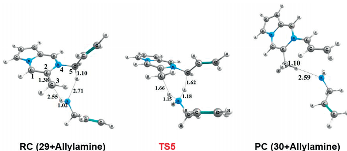
Figure 7. Optimized geometries of the stationary points of the formation of 30 at CPCM/B3LYP/6-31+G(d,p)//B3LYP/6-31+G(d,p) level in methanol. Distances are given in angstroms.
