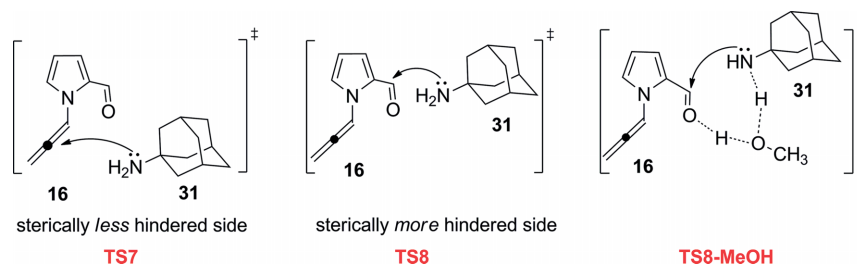
Scheme 11. Possible transition states for the reaction of 16 with 31 .
