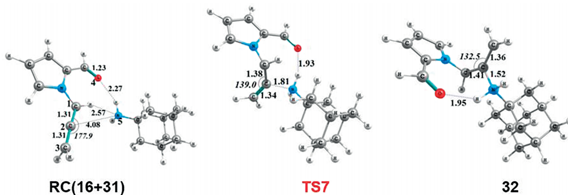
Figure 9. Optimized geometries of the stationary points of the first step for the formation of 32 at CPCM/B3LYP/6-31+G(d,p)//B3LYP/6-31+G(d,p) level in methanol. Distances are given in angstroms, angles are given in degrees.
