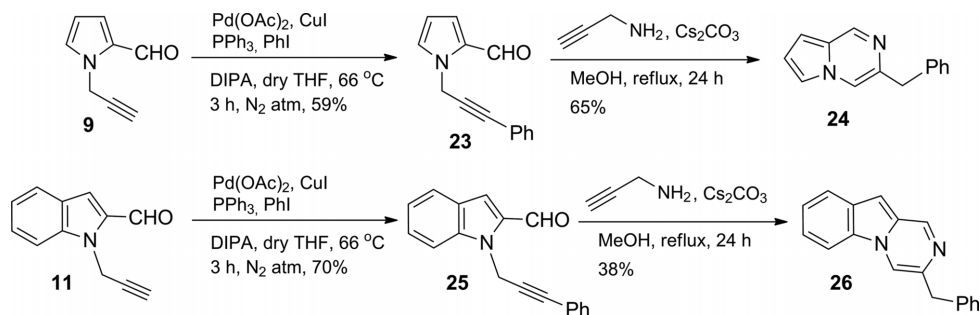
Scheme 9. Synthesis of 23 and 25 and their reaction with propargylamine to give 24 and 26 .
