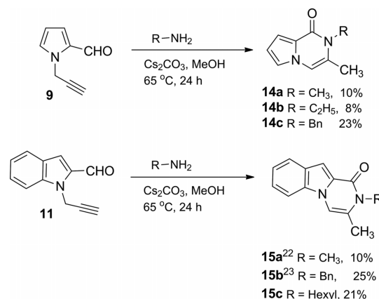
Scheme 3. Formation of pyrrolo- and indolo-pyrazinones 14 and 15 .
