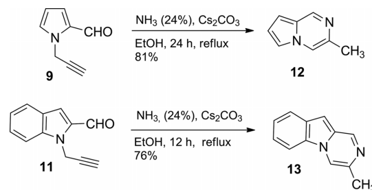
Scheme 2. Cyclization of N -propargylated pyrrole- and indole-2-carbaldehyde with ammonia.
