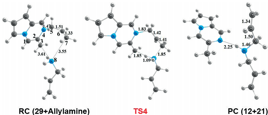
Figure 6. Optimized geometries of the stationary points of the path 2 at CPCM/B3LYP/6-31+G(d,p)//B3LYP/6-31+G(d,p) level in methanol. Distances are given in angstroms.
