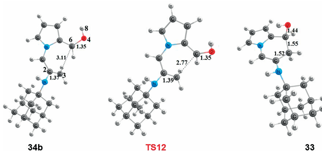
Figure 13. Optimized geometries of the stationary points for the formation of 33 at CPCM/B3LYP/6-31+G(d,p)//B3LYP/6-31+G(d,p) level in methanol. Distances are given in angstroms.
