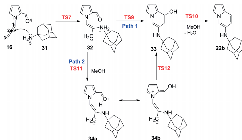
Scheme 12. Proposed mechanisms for the formation of 22b .
