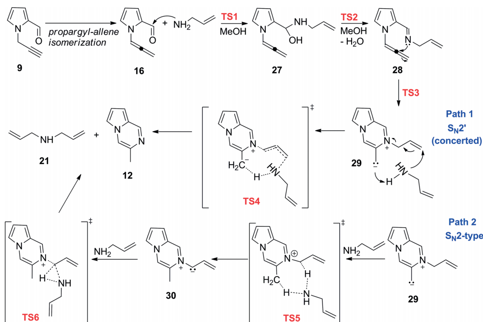
Scheme 10. Possible pathways for the formation of 12 . Path 2 is the preferred path as revealed by DFT calculations.
