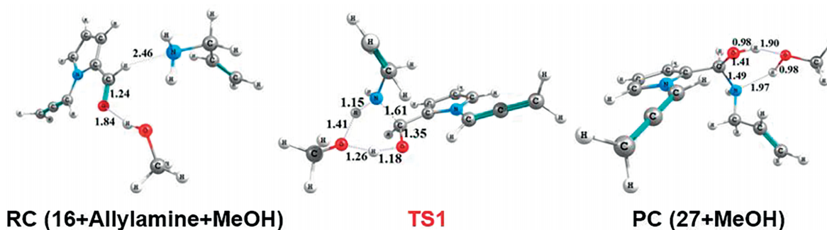
Figure 3. Optimized geometries for the stationary points for the formation of hemiaminal 27 at CPCM/B3LYP/6-31+G(d,p)//B3LYP/6-31+G(d,p) level in methanol. Distances are given in angstroms.
