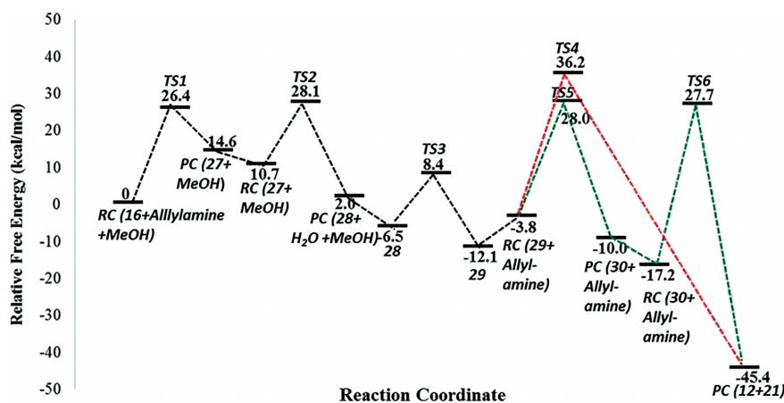
Figure 2. Potential energy profile and relative Gibbs free energies (kcal/mol) in methanol related to the formation of pyrrolo-pyrazine derivative 12 at CPCM/B3LYP/6-31+G(d,p)//B3LYP/6-31+G(d,p) level. Black, common steps; red, path 1; green, path 2.
