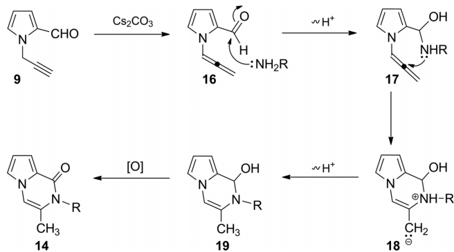
Scheme 4. Proposed mechanism for the formation of 14 (and 15 ).
