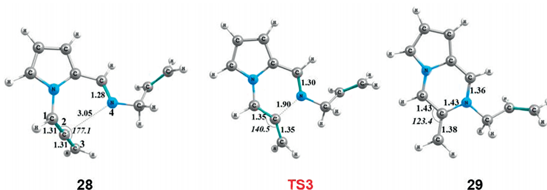
Figure 5. Optimized geometries of the stationary points for the formation of 29 at CPCM/B3LYP/6-31+G(d,p)//B3LYP/6-31+G(d,p) level in methanol. Distances are given in angstroms; angles are in degrees.
