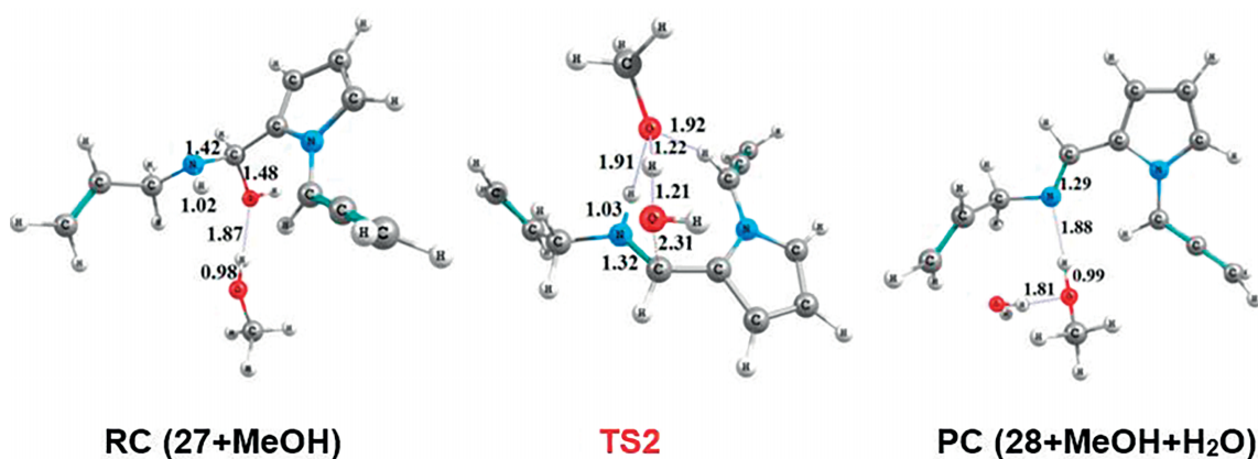
Figure 4. Optimized geometries for the stationary points for the formation of imine 28 at CPCM/B3LYP/6-31+G(d,p)//B3LYP/6-31+G(d,p) level in methanol. Distances are given in angstroms.
