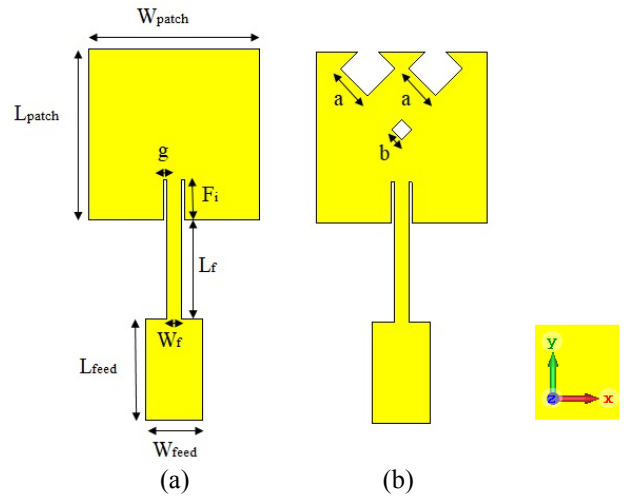
Figure 1. (a) Conventional square patch antenna, (b) Proposed square patch antenna with diamond – shaped slots.
