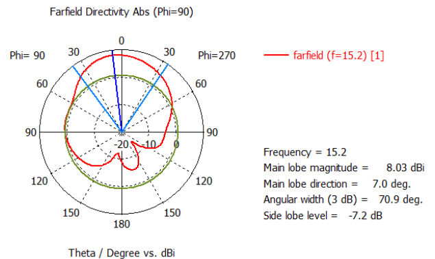
Figure 6. Radiation patterns for the square patch antenna with diamond – shaped slots on the radiating part.
