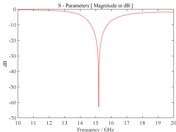
Figure 4. Return loss plot versus frequency for the square patch antenna with diamond – shaped defect on the ground plane.
