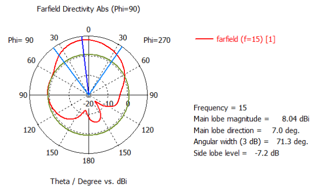
Figure 5. Radiation patterns for the conventional square patch antenna.
