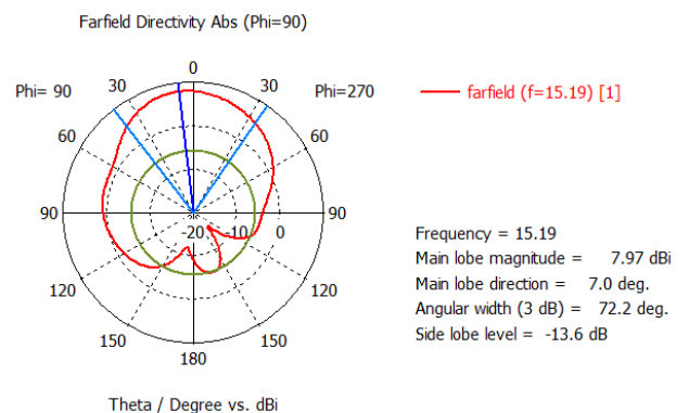
Figure 7. Radiation patterns for the square patch antenna with diamond – shaped slots on the radiating part and with defected ground.
