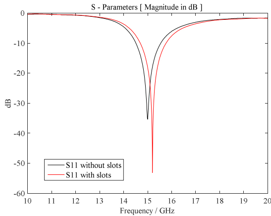
Figure 2. Return loss plot versus frequency for the conventional square patch antenna and for the square patch antenna with diamond – shaped slots.
