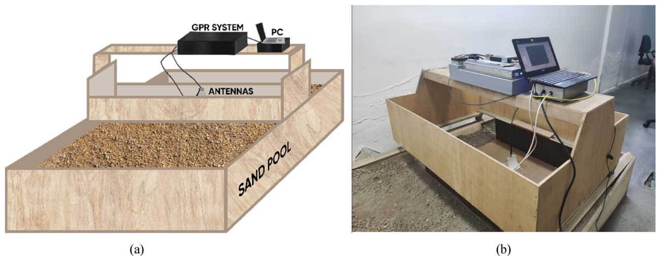
Figure 12. (a) Configuration of the measurement setup and (b) the picture of the measurement environment utilized to generate experimental data set for the use of proposed customized deep learning based surrogate model.
